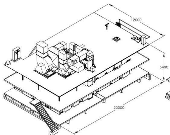
TOP DECK
